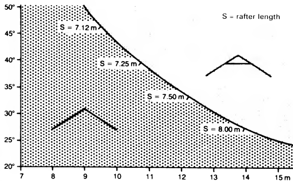
① Economic limits, slope v. span: couple/collar roofs
